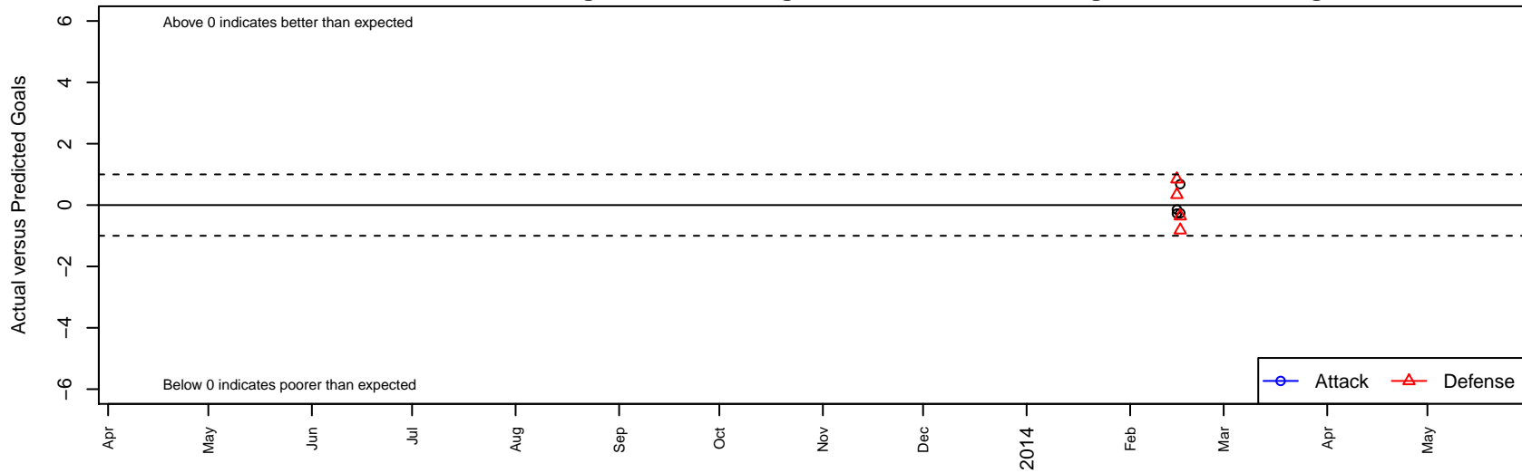
AUFC 96 NM B95 Dots are actual minus expected GF (blue circles) and GA (red triangles). Blue line is smoothed change in attack strength. Red is smoothed change in defense strength.
